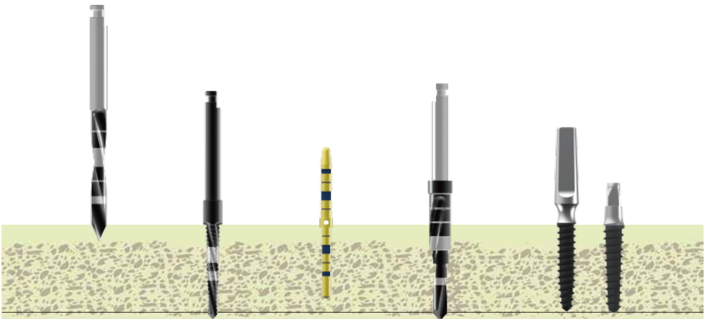
Guide Drill Lindemann Drill Parallel Pin Step Drill Ø3.0 Implant
